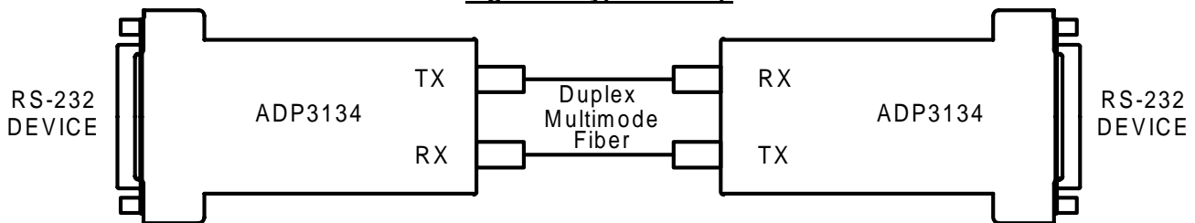
Figure 2: Typical Setup
